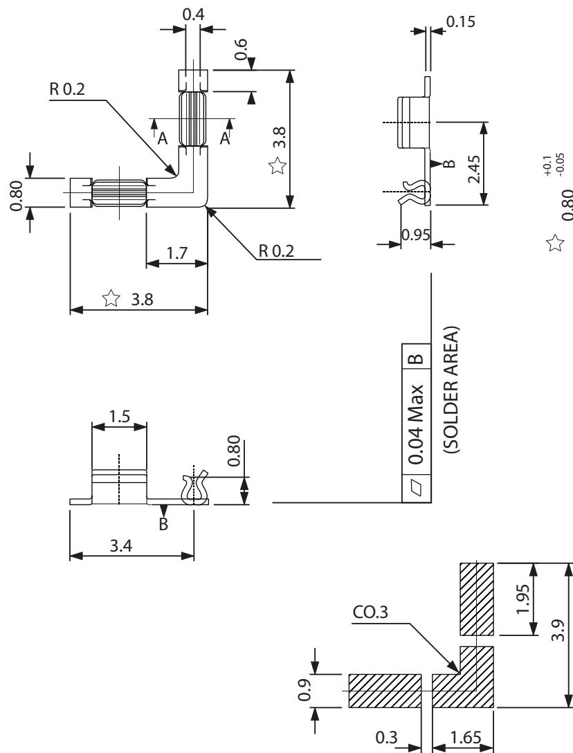
Soldering Land Pattern 0.1T
